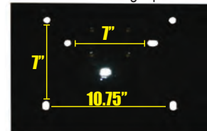
Bottom View Various Mounting Options
