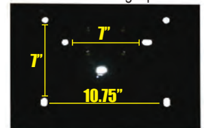
Bottom View Various Mounting Options
